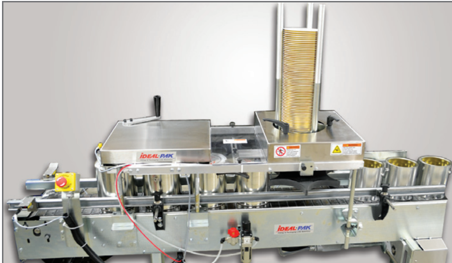
Ideal-Pak Model LPA-0000 Automatic Lid Placer shown with optional Ideal-Pak 2340 HR Roller Closing Machine and Conveyor.
